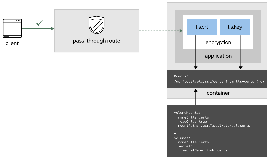
Figure 5.7: Securing applications with passthrough routes
