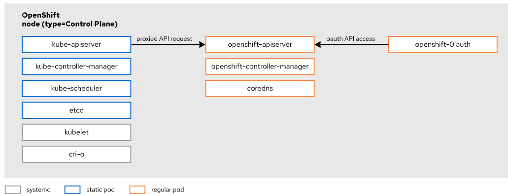
Figure 1.3: Architecture of an OpenShift control plane node
