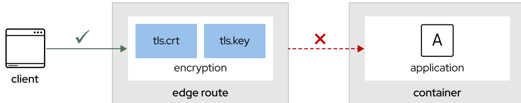
Figure 5.6: Securing applications with edge routes
